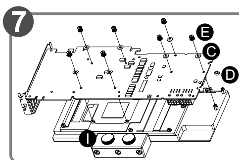
When installing the water block, carefully position the water block with the preinstalled standoffs on the graphics card.
