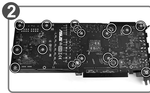
Remove the screws circled on the diagram. All heat sink assembly screws should be removed.
