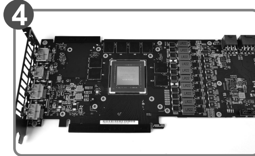
Clean the original thermal compound off the GPU die
