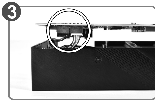
Remove the power connector (Carefully detach the original stock cooler)
